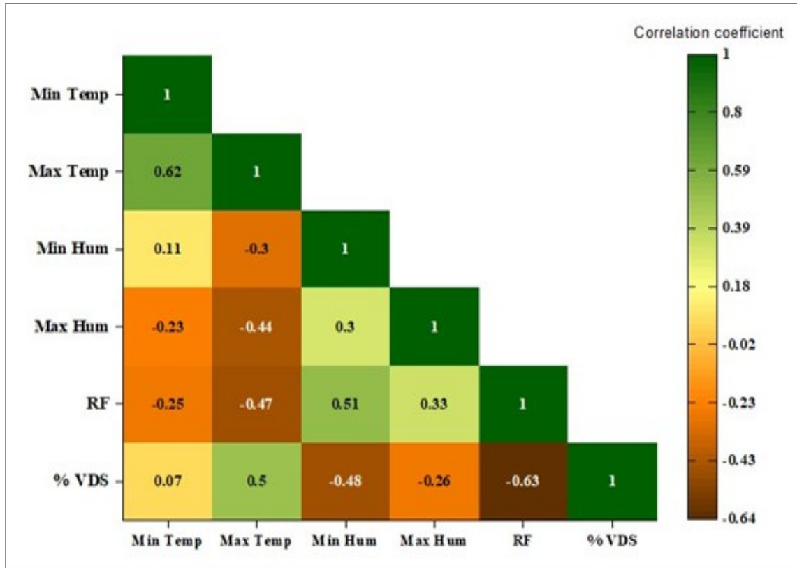
Fig. 8. Heat map correlation (Pearson correlation) on influence of weather factors with % vines damaged by scales (% VDS) and the results of the correlation analysis have been scaled by a color gradient that goes from green (positive correlation) to dark orange (negative correlation) by increasing color density, significant correlation coefficients at p \leq 0.05 , ** p \leq 0.01 , and *** p \leq 0.001 .
