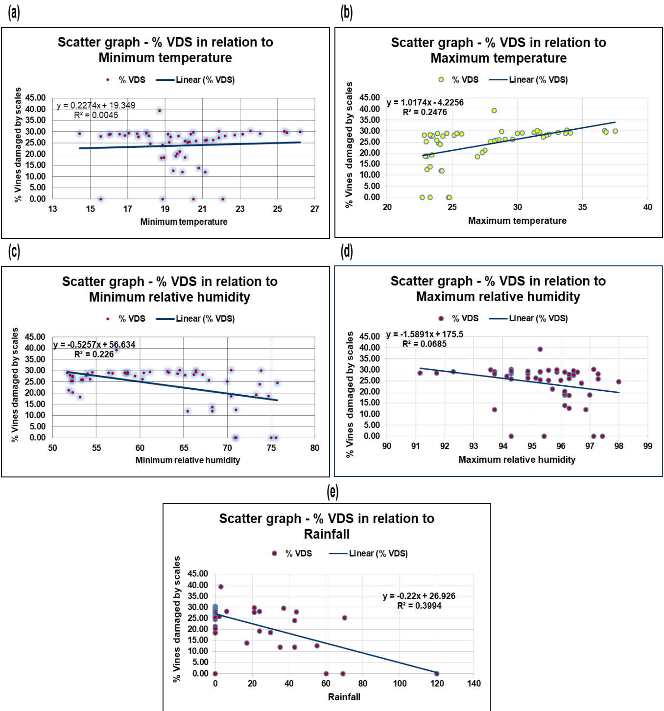
Fig. 9. Scatter graph of % vine damaged by scales (% VDS) in relation to weather factors (a) Minimum temperature (b) Maximum temperature (c) Minimum humidity (d) Maximum humidity (e) Rainfall.
