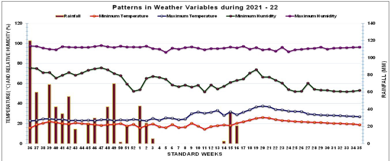
Fig. 1. Patterns in the weather variables during 2021 - 22.
