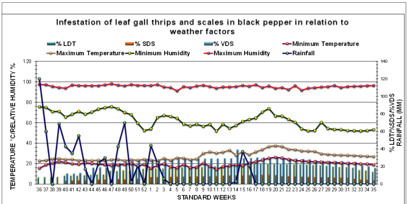
Fig. 2. Population dynamics of leaf gall thrips, scales in relation to weather factors.
