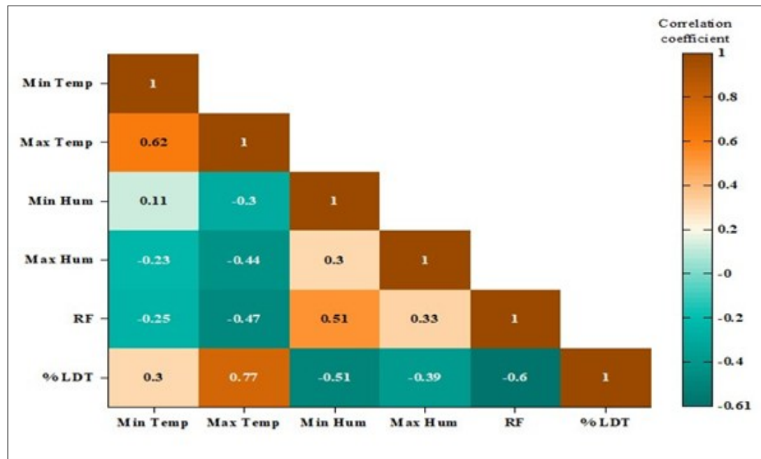
Fig. 4. Heat map correlation (Pearson correlation) on influence of weather factors with % leaves damaged by thrips (% LDT) and the results of the correlation analysis have been scaled by a color gradient that goes from dark brown (positive correlation) to light blue (negative correlation) by increasing color density, significant correlation coefficients at p \leq 0.05 , ** p \leq 0.01 and *** p \leq 0.001 .
