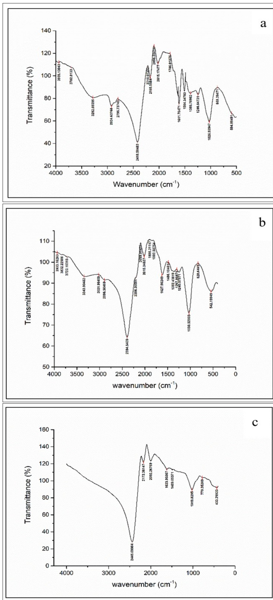
Fig. 2. FT-IR spectral graph of T. ulmifolia plant parts; a) Leaf b) stem c) root.
