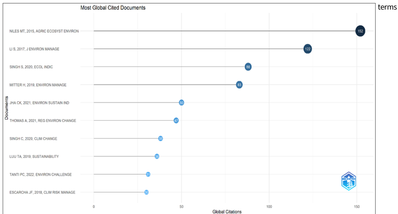
Fig. 5. Most global cited articles (R studio).
