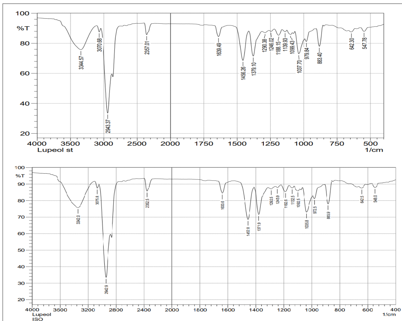
Fig. 4. FT-IR spectra of isolated lupeol and lupeol standard.
