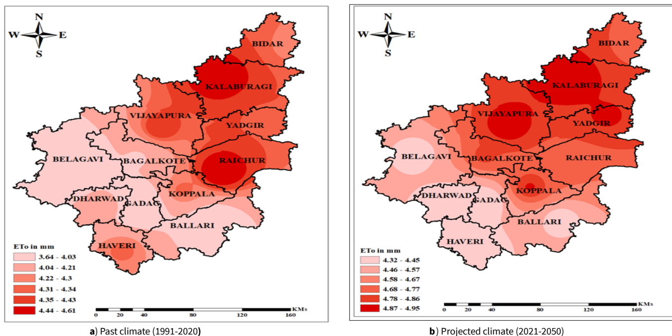
Fig. 2. Spatial distribution of Reference Evapotranspiration ( ET_o ) (mm day -1 ) under both past (1991-2020) and projected (2021-2050) climatic scenarios for soybean crop duration (June-September) across NIK.
